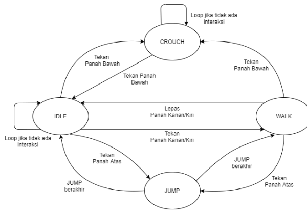
Gambar. 3. FSM player
