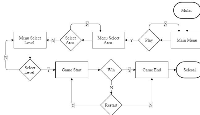
Gambar. 1. Flowchart
