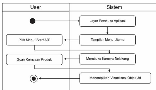
Gambar 5. Activity Diagram
