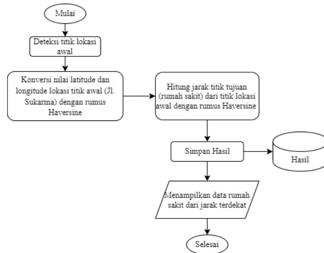
Gambar. 2. Flow Chart Metode Haversine
