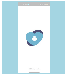
Gambar. 4. Splash Screen
