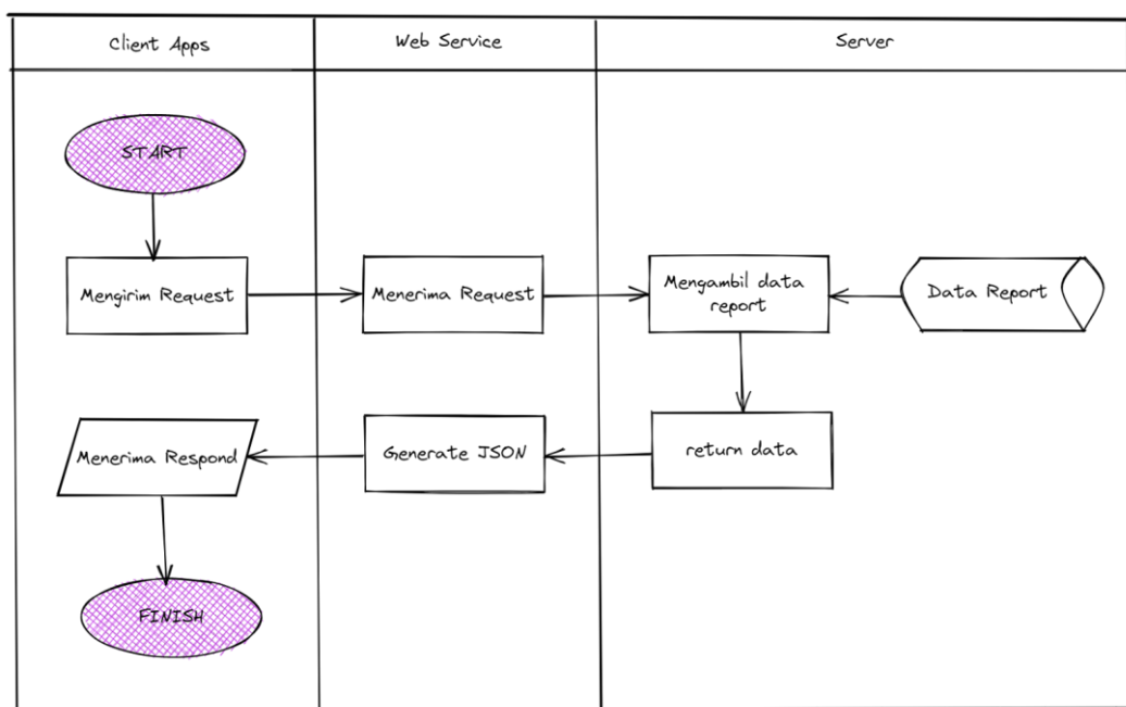
Gambar 2. Flowchart GET
