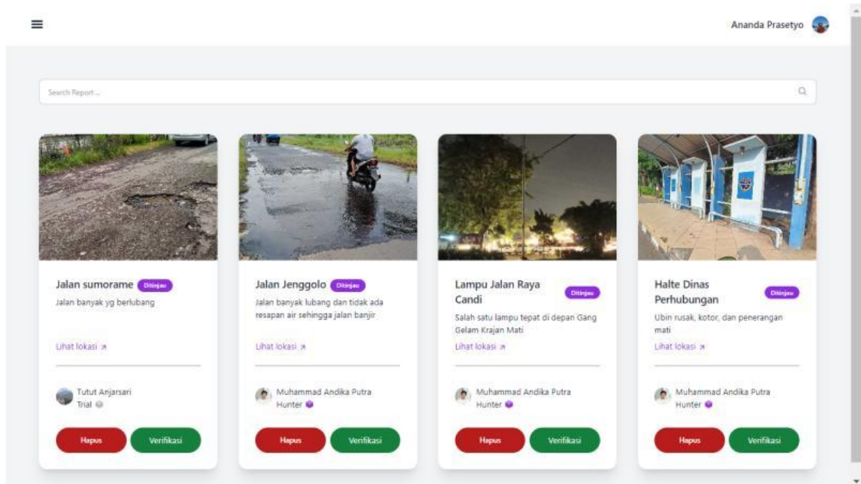
Gambar 8. Halaman Report
