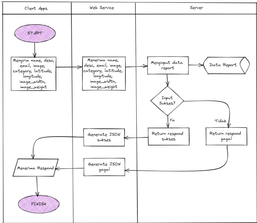
Gambar 3. Flowchart POST
