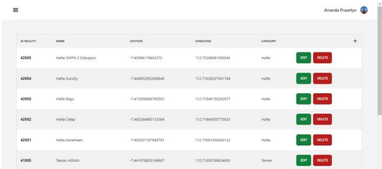
Gambar 10. Halaman Facility
