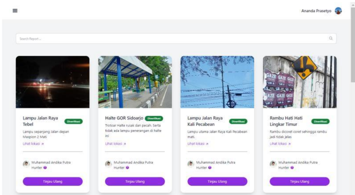
Gambar 9. Halaman History
